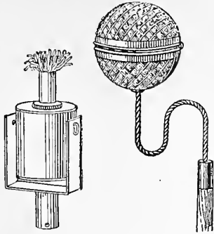
Reservoir Torch Asbestos Torch
